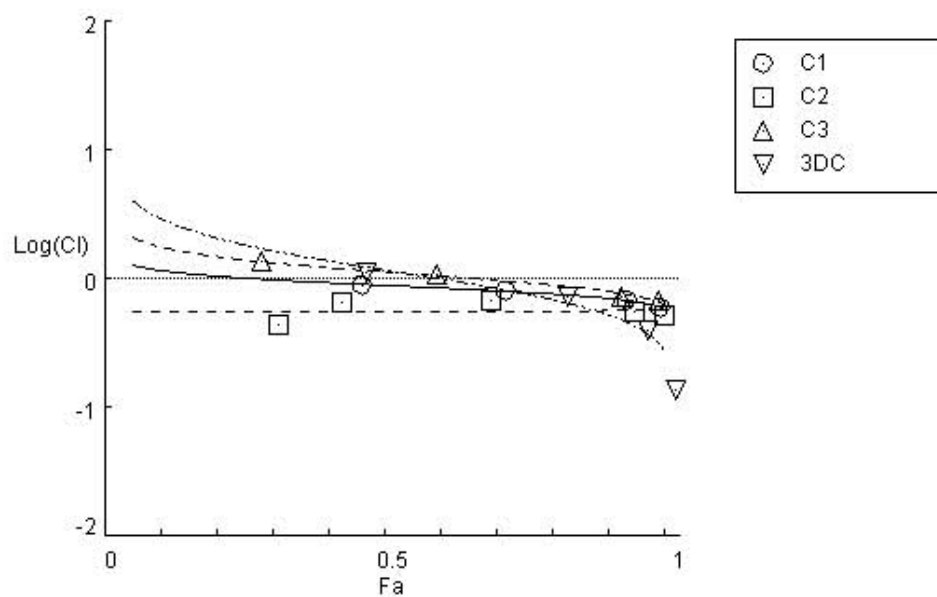
Figure 4.2: An Example F_a - \text{Log}(CI) Plot.
