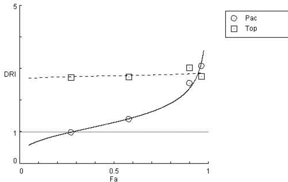
Figure 4.4: An Example Fa - DRI Plot.
