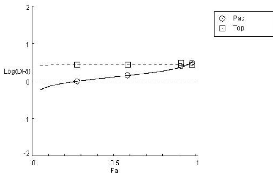
Figure 4.5: An Example F_a -Log(DRI) Plot.
