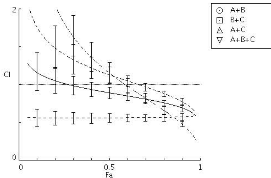
Figure 4.7: An Example F_\alpha -CI Plot with Sequential Deletion Analysis.
